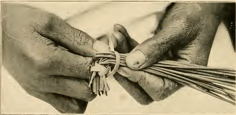
FIG. 10. THE SECOND LOOP OF THE THREAD TOO FAR FROM THE FIRST MAKING THE COIL CURVE TOO ABRUPTLY.
